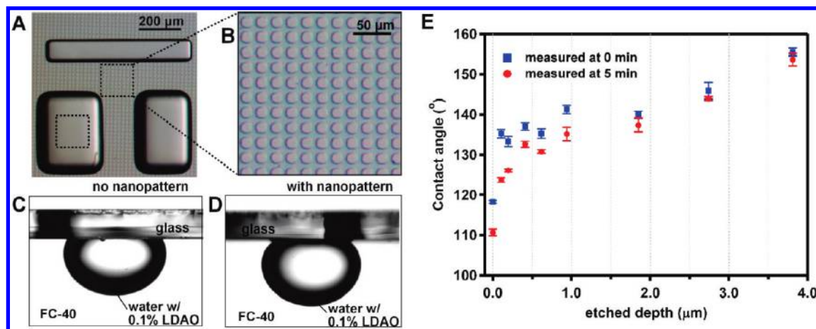
Figure 5. Patterning hydrophobicity on the surface of the SlipChip with nanometer deep micropatterns. (A) Microphotograph of the surface of the SlipChip after nanopatterning. No nanopatterning is present on the surface of the wells or microchannels. (B) Zoomed-in microphotograph shows the surface patterning of small wells 10 \mu\text{m} in diameter and 250 nm deep. (C) Microphotograph of a 4- \mu\text{L} aqueous droplet deposited on a surface silanized without nanopatterning. The droplet contained 0.1% (w/v) LDAO. The contact angle was measured right after the deposition and was 115.4°. (D) Microphotograph of a 4- \mu\text{L} aqueous droplet deposited on a surface silanized with nanopatterning of 250 nm depth. The droplet contained 0.1% (w/v) LDAO. The contact angle was measured right after the deposition and was 137.9°. (E) Contact angle of a 0.1% LDAO solution on silanized glass with different nanopatterns. The nanopatterns were obtained with the same nanopatterning photomask used to construct the SlipChips with nanopatterning (10 \mu\text{m} size cross mesh with 10 \mu\text{m} spacing), but different nanowell depths were obtained by changing the etching time. The contact angle was measured immediately after the droplet was deposited on the glass plate (at 0 min) and again 5 min after the deposition.
