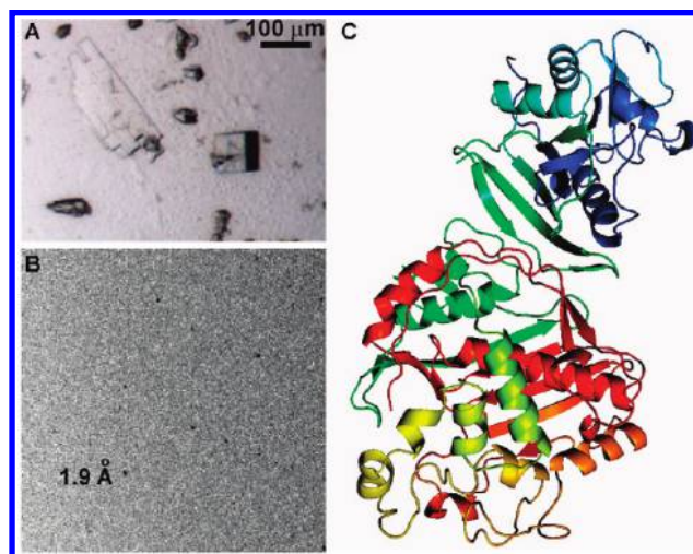
Figure 7. Determination of the crystal structure of dihydrofolate reductase/thymidylate synthase (PDBid: 3KJR). (A) A microphotograph of crystals of dihydrofolate reductase/thymidylate synthase grown in scale-up experiments performed in well plates, by using the exact condition recognized in a microbatch SlipChip, at a mixing ratio of 0.33:0.67 with 20% (w/v) PEG-8000, 0.2 M NaCl and 0.1 M CHES, pH 9.5. (B) An X-ray diffraction pattern obtained from crystals in A at a region of 1.9 Å resolution. (C) Structure of dihydrofolate reductase/thymidylate synthase (refined to 1.95 Å resolution) obtained from crystals grown in scale-up experiments. The structure is displayed in cartoon generated using Pymol.
